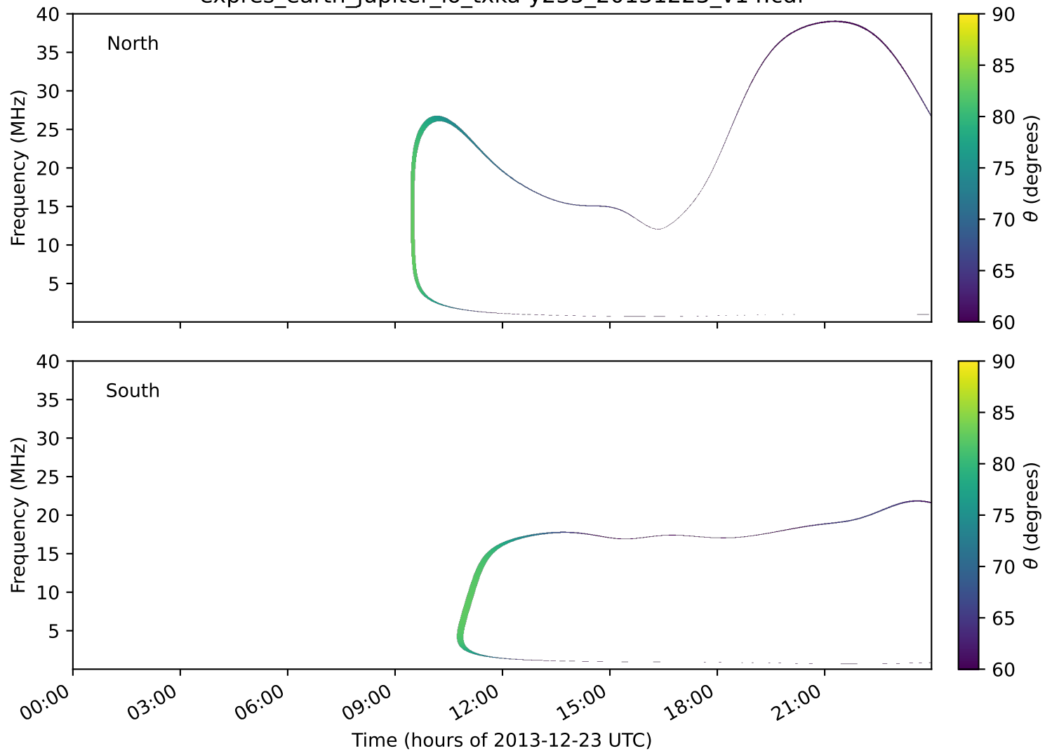
expres_earth_jupiter_io_txka-y235_20131223_v14.cdf
