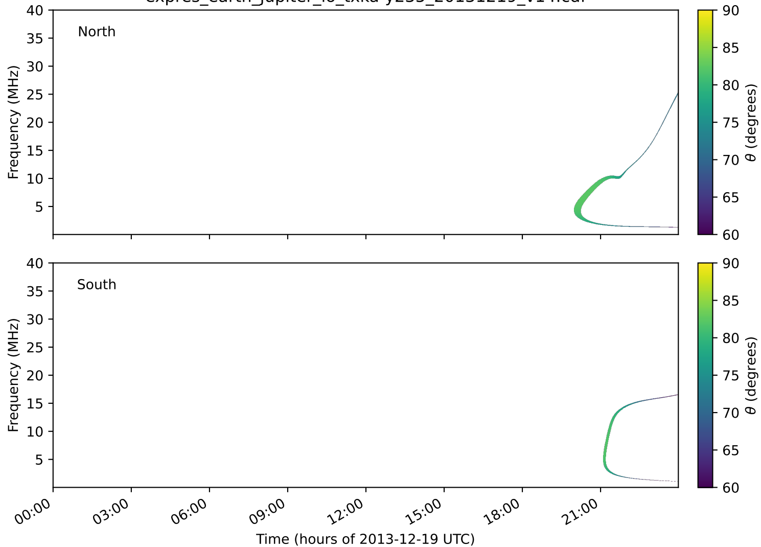
expres_earth_jupiter_io_txka-y235_20131219_v14.cdf
