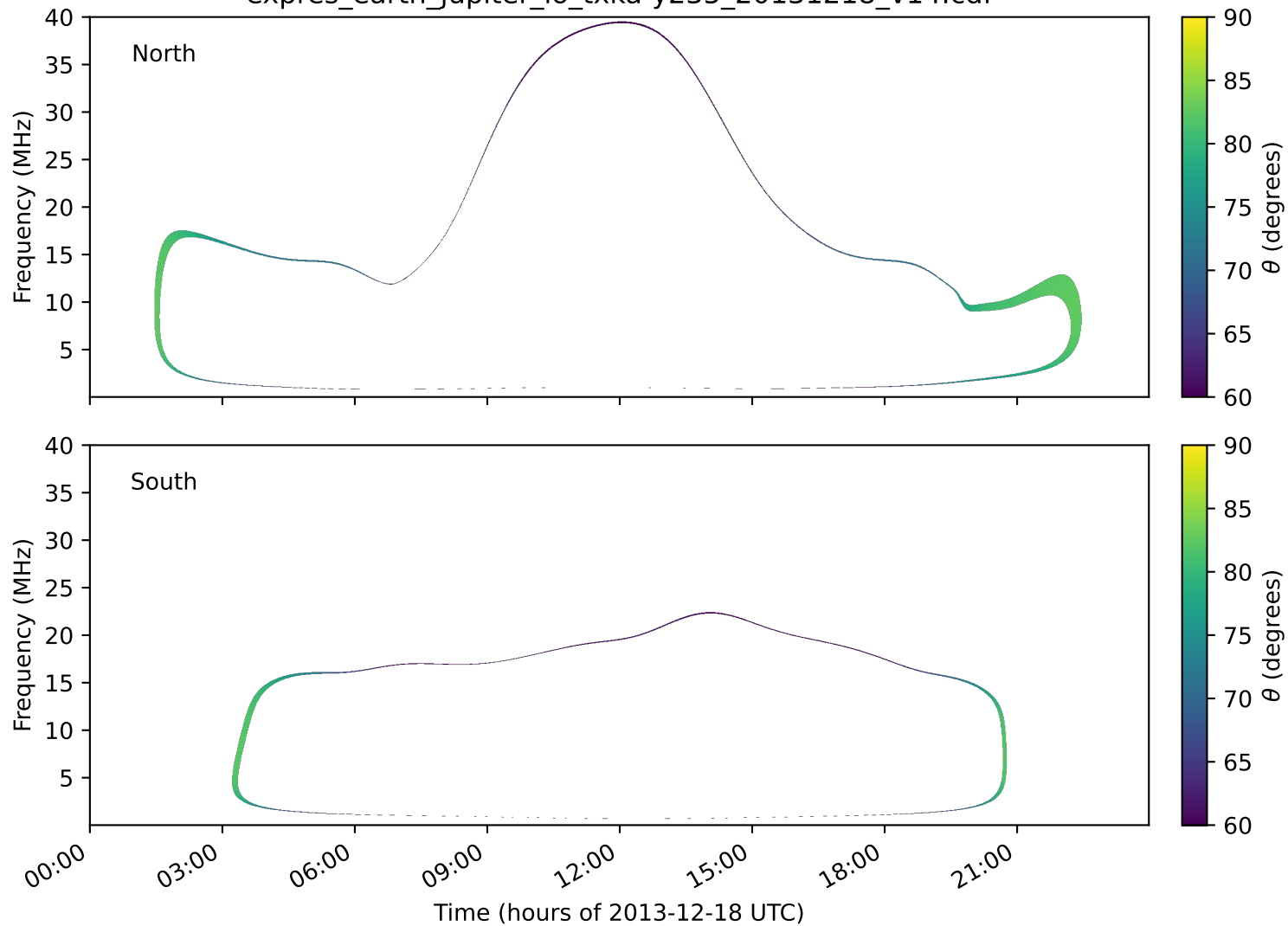
expres_earth_jupiter_io_txka-y235_20131218_v14.cdf
