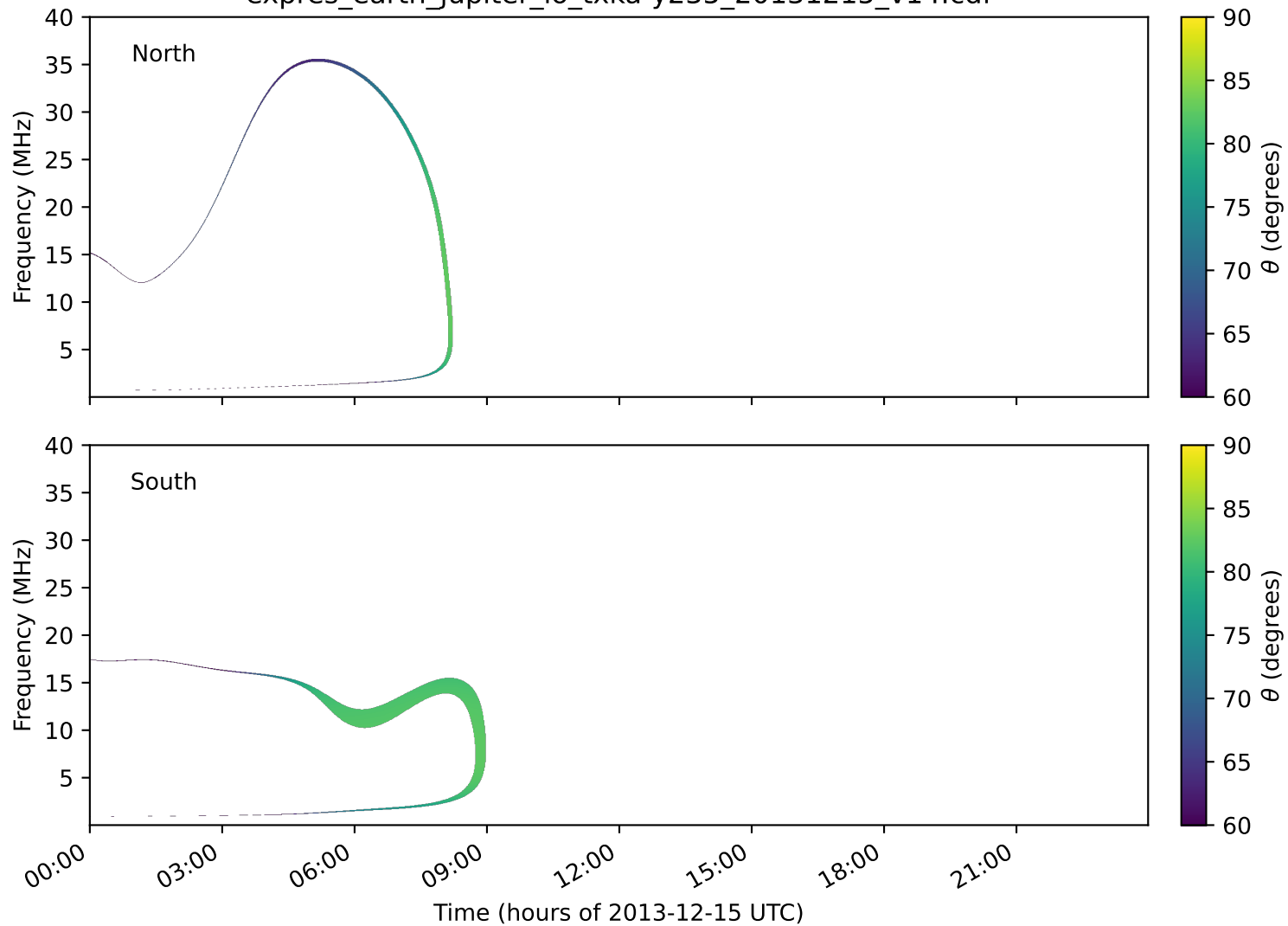
expres_earth_jupiter_io_txka-y235_20131215_v14.cdf
