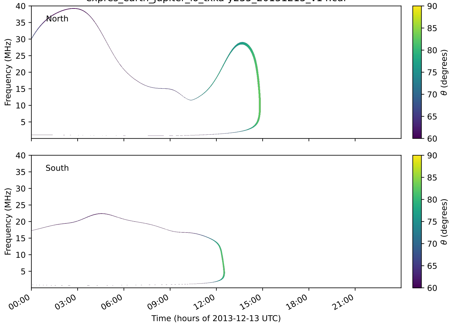
expres_earth_jupiter_io_txka-y235_20131213_v14.cdf
