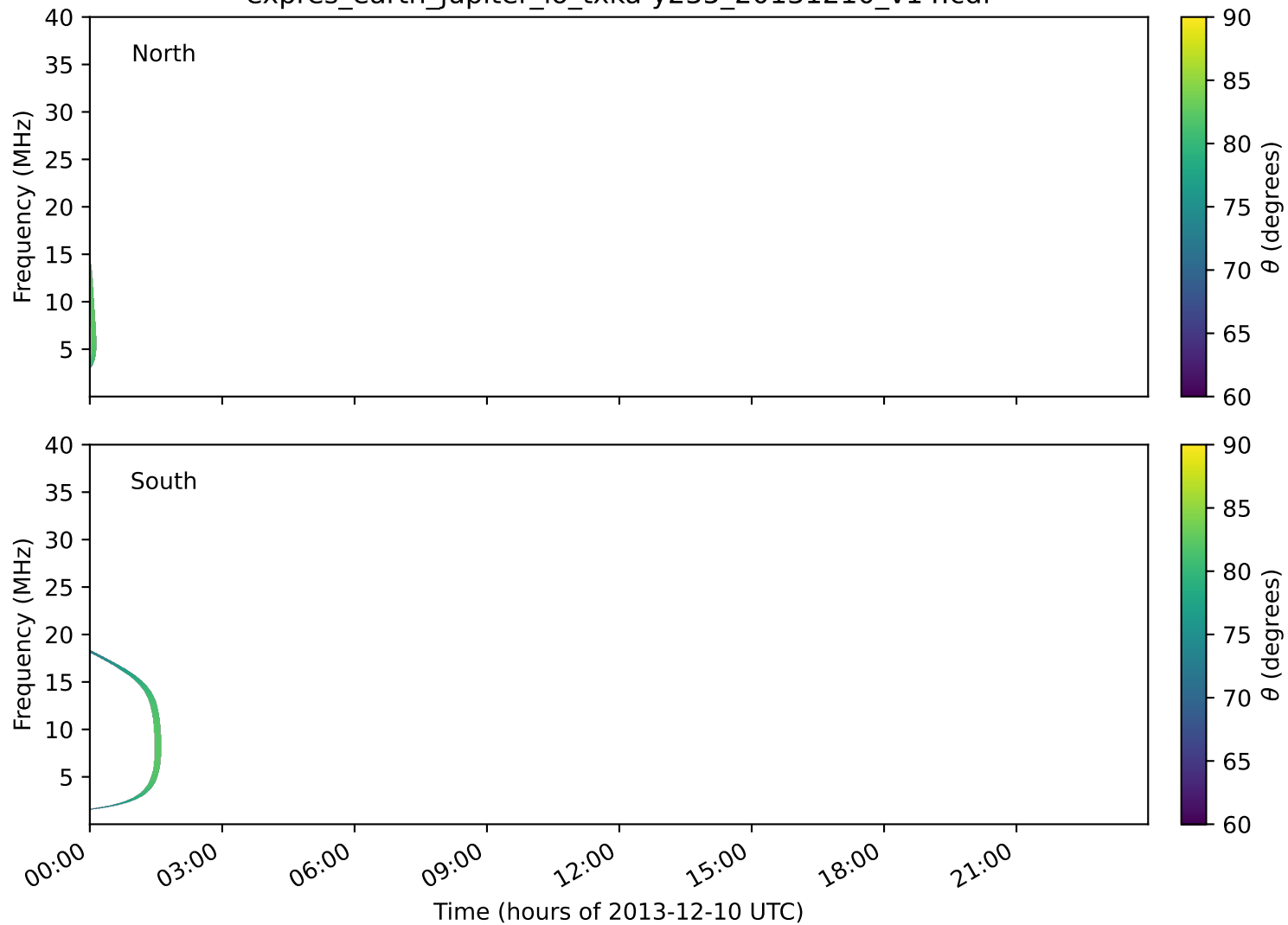
expres_earth_jupiter_io_txka-y235_20131210_v14.cdf
