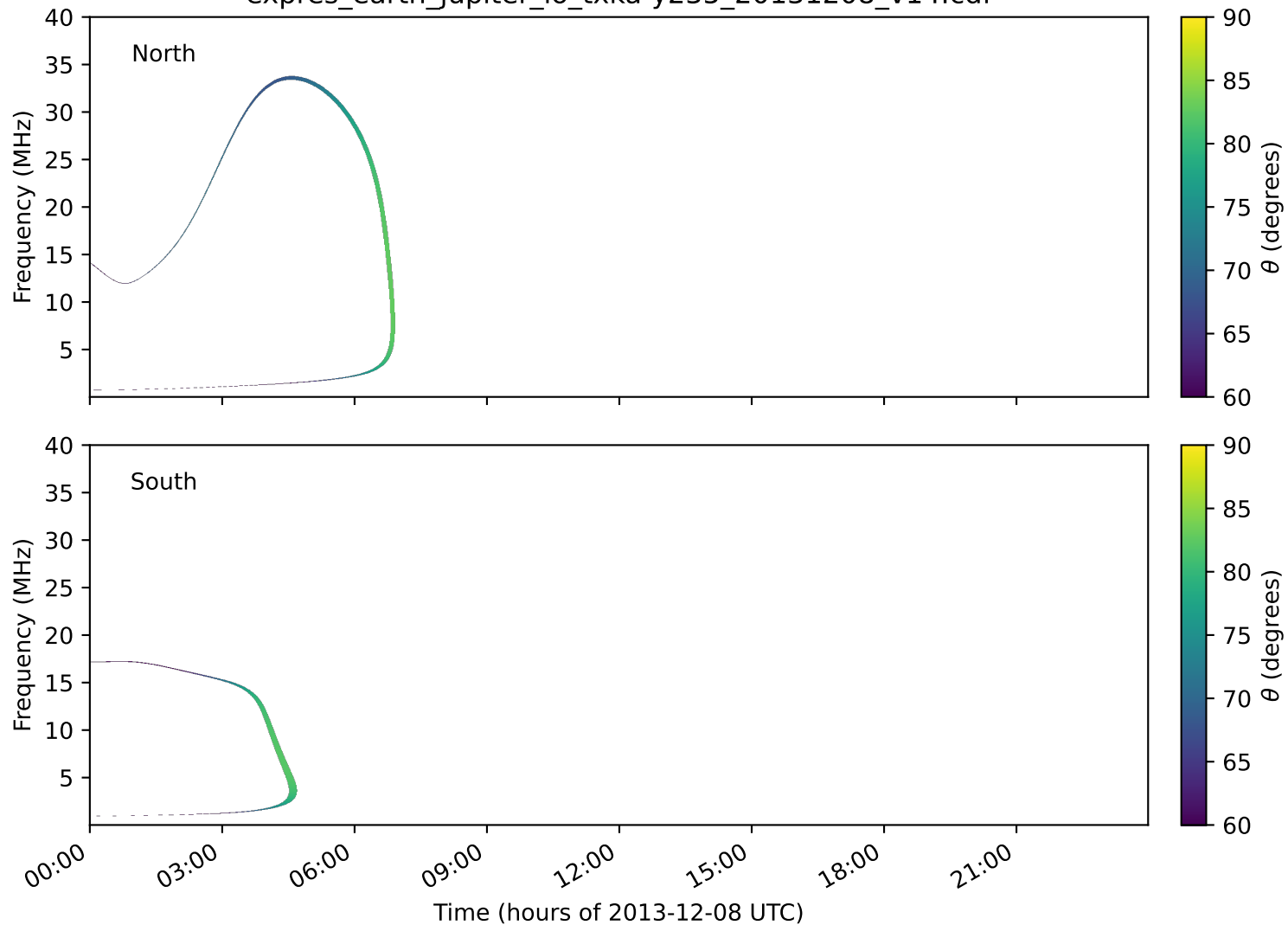
expres_earth_jupiter_io_txka-y235_20131208_v14.cdf
