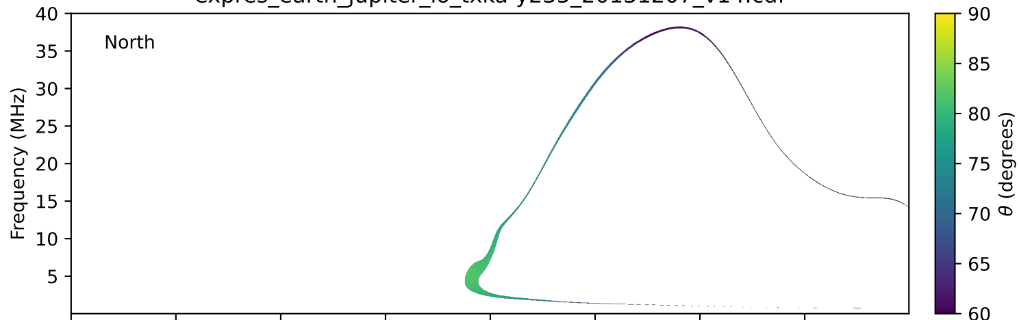
expres_earth_jupiter_io_txka-y235_20131207_v14.cdf
