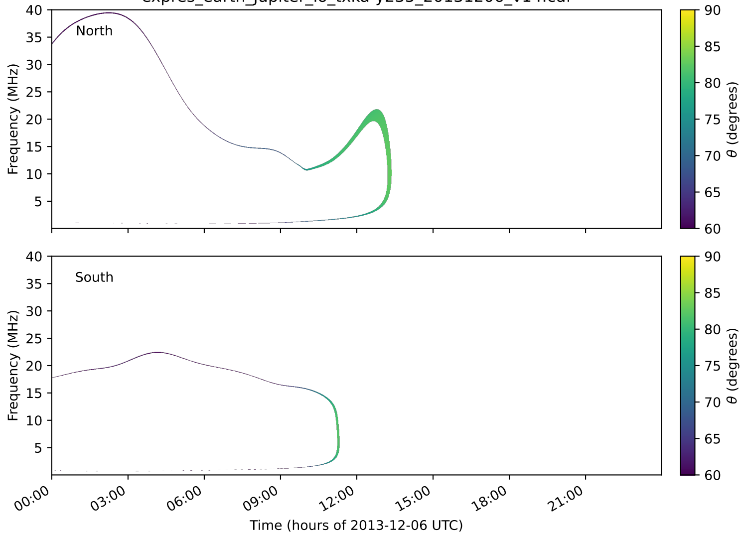
expres_earth_jupiter_io_txka-y235_20131206_v14.cdf
