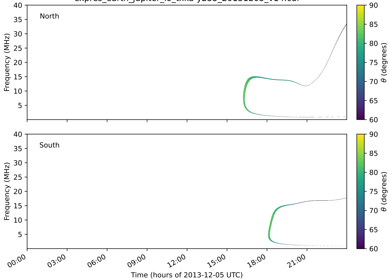
expres_earth_jupiter_io_txka-y235_20131205_v14.cdf
