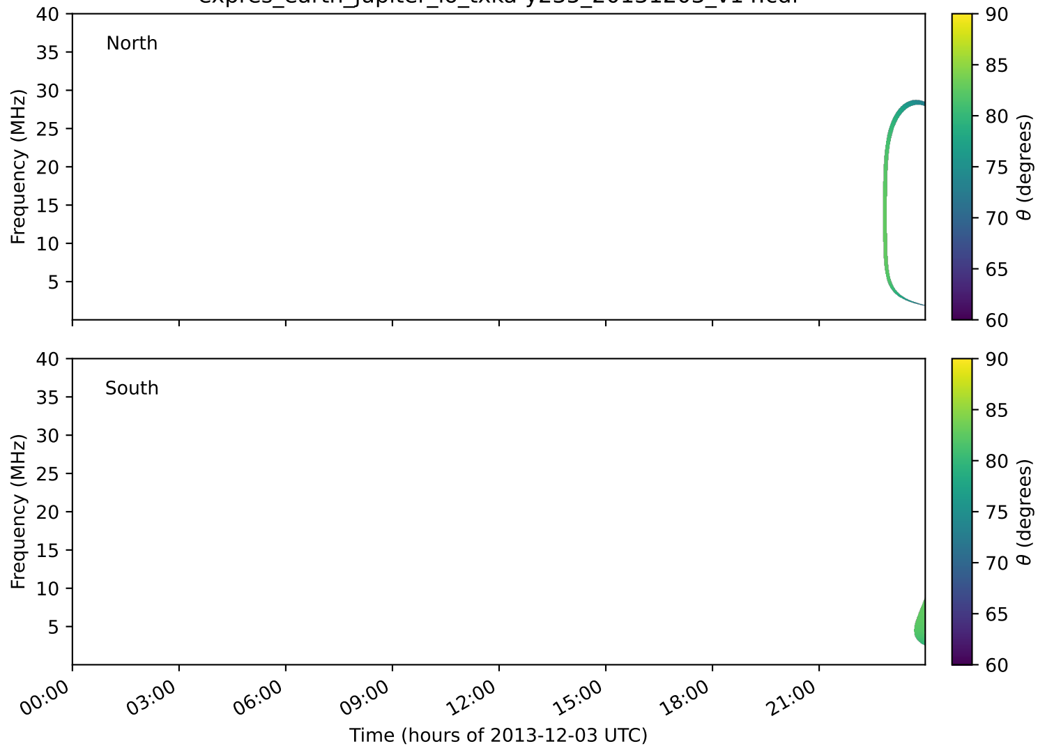
expres_earth_jupiter_io_txka-y235_20131203_v14.cdf
