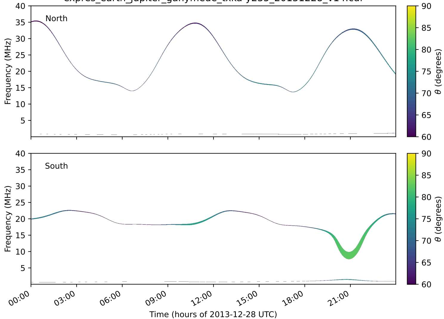
expres_earth_jupiter_ganymede_txka-y235_20131228_v14.cdf
