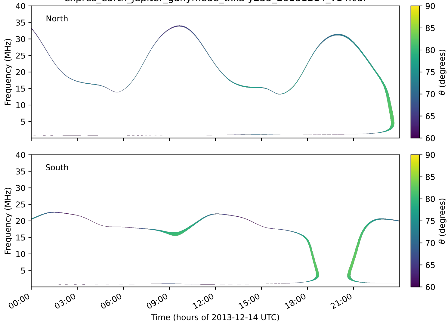
expres_earth_jupiter_ganymede_txka-y235_20131214_v14.cdf
