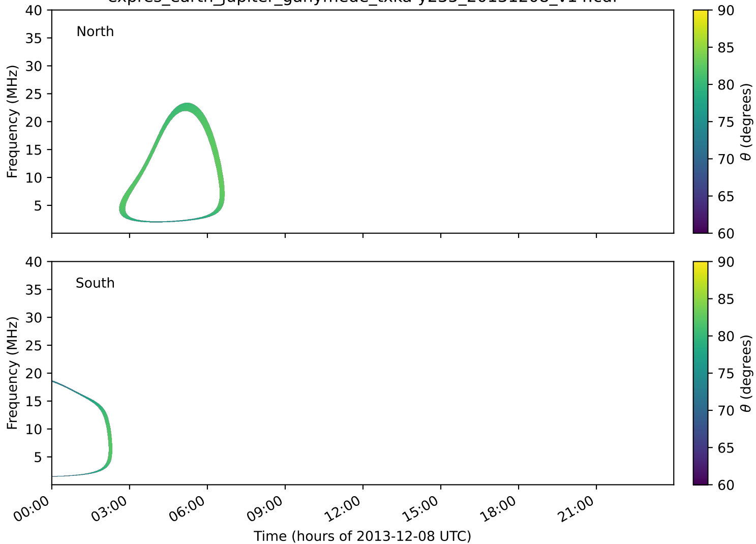
expres_earth_jupiter_ganymede_txka-y235_20131208_v14.cdf
