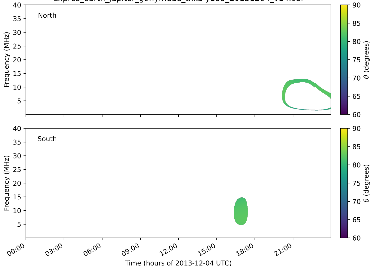
expres_earth_jupiter_ganymede_txka-y235_20131204_v14.cdf
