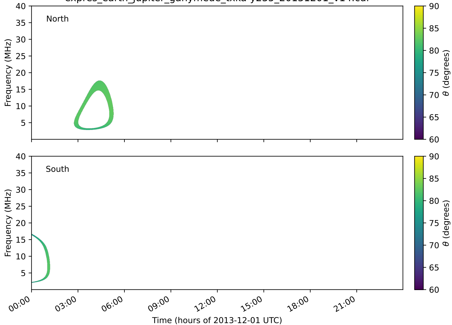
expres_earth_jupiter_ganymede_txka-y235_20131201_v14.cdf
