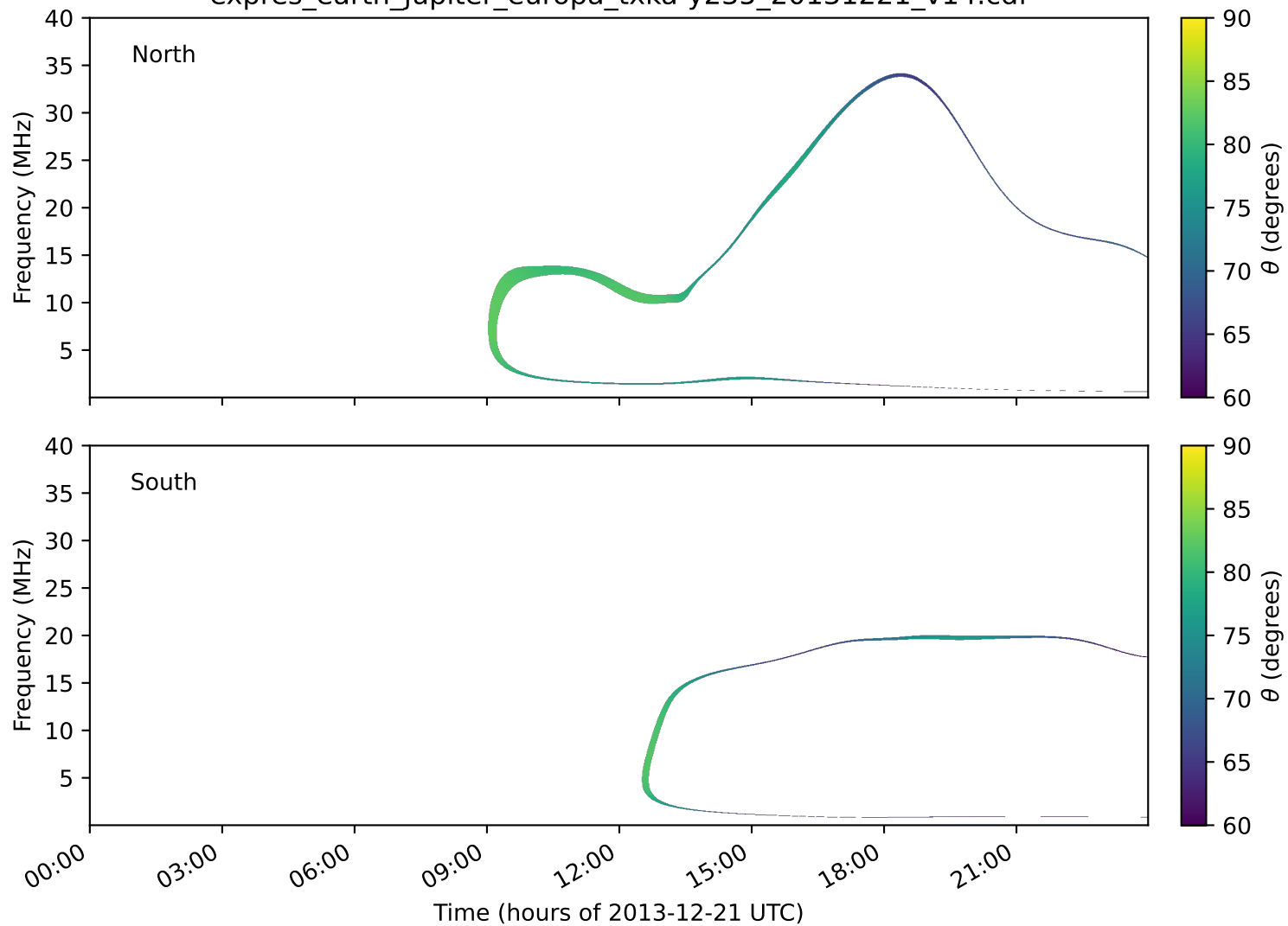
expres_earth_jupiter_europa_txka-y235_20131221_v14.cdf
