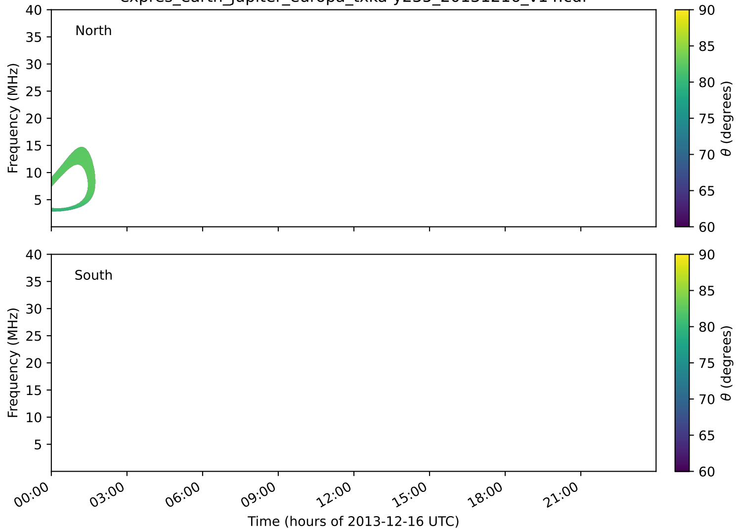
expres_earth_jupiter_europa_txka-y235_20131216_v14.cdf
