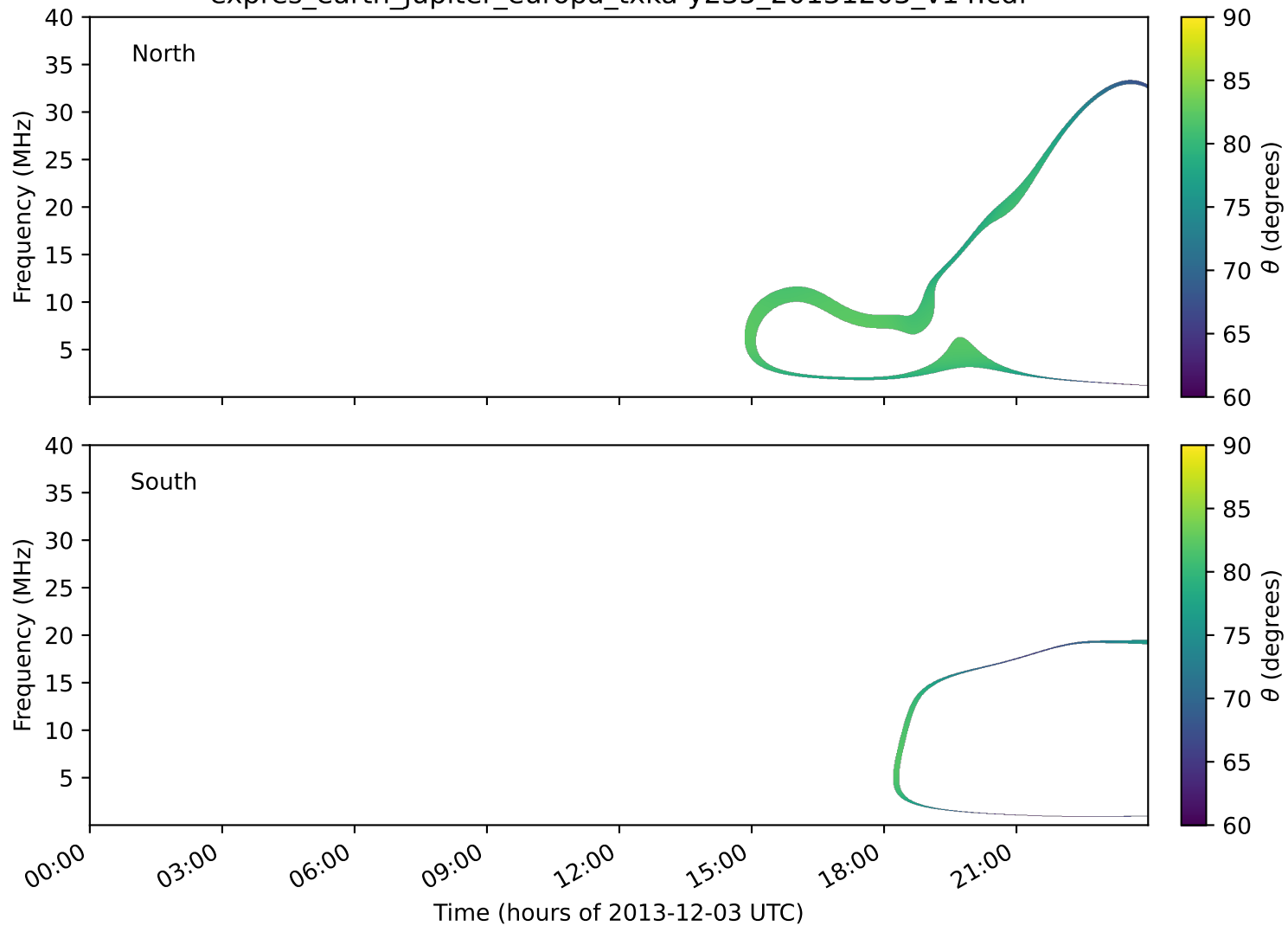
expres_earth_jupiter_europa_txka-y235_20131203_v14.cdf
