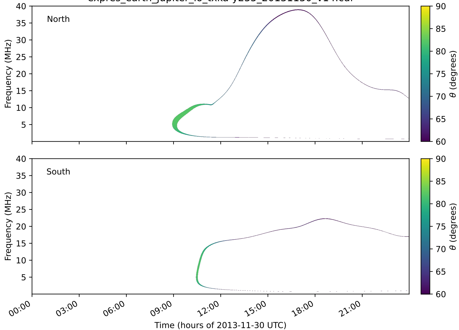
expres_earth_jupiter_io_txka-y235_20131130_v14.cdf
