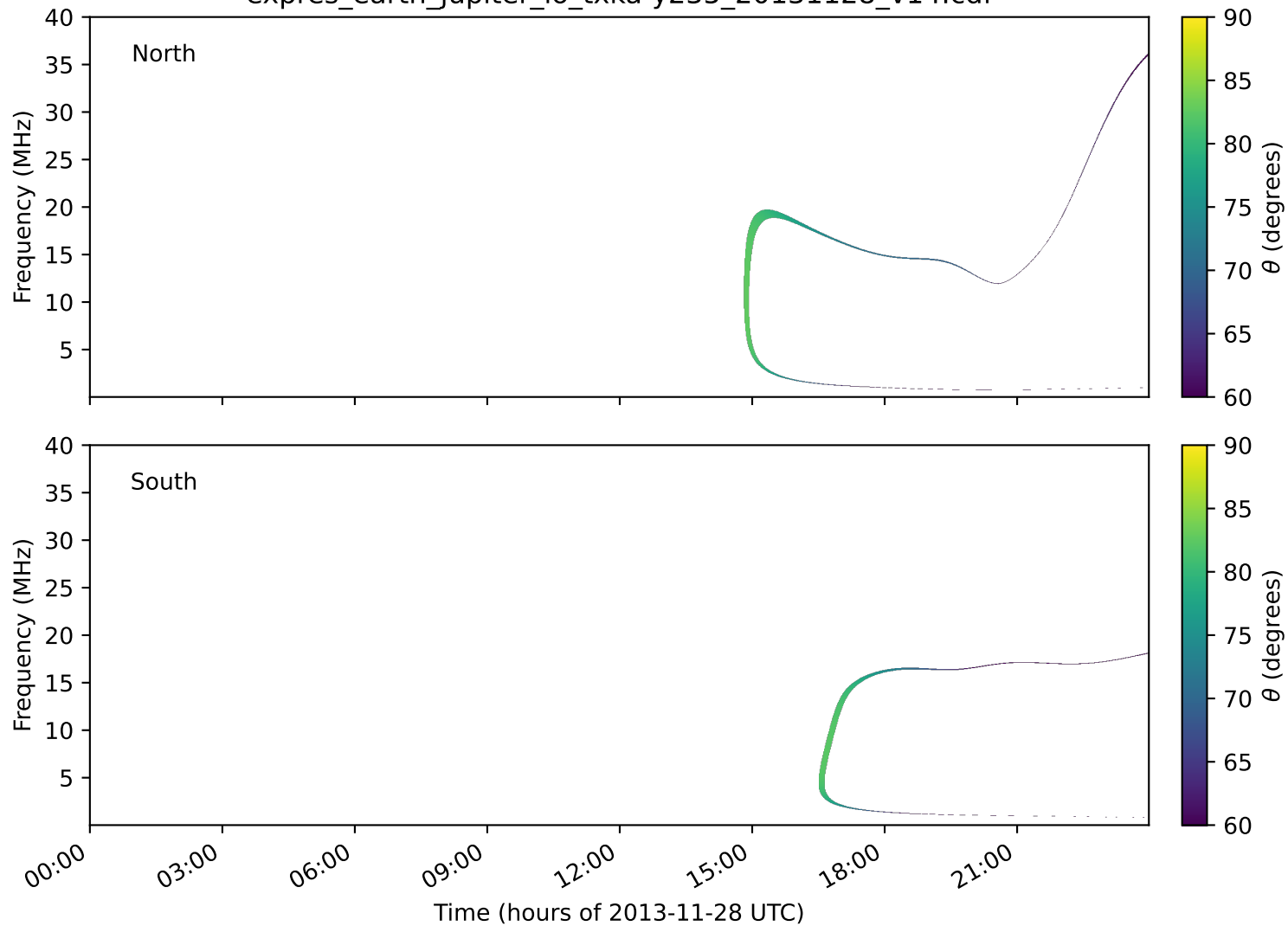
expres_earth_jupiter_io_txka-y235_20131128_v14.cdf
