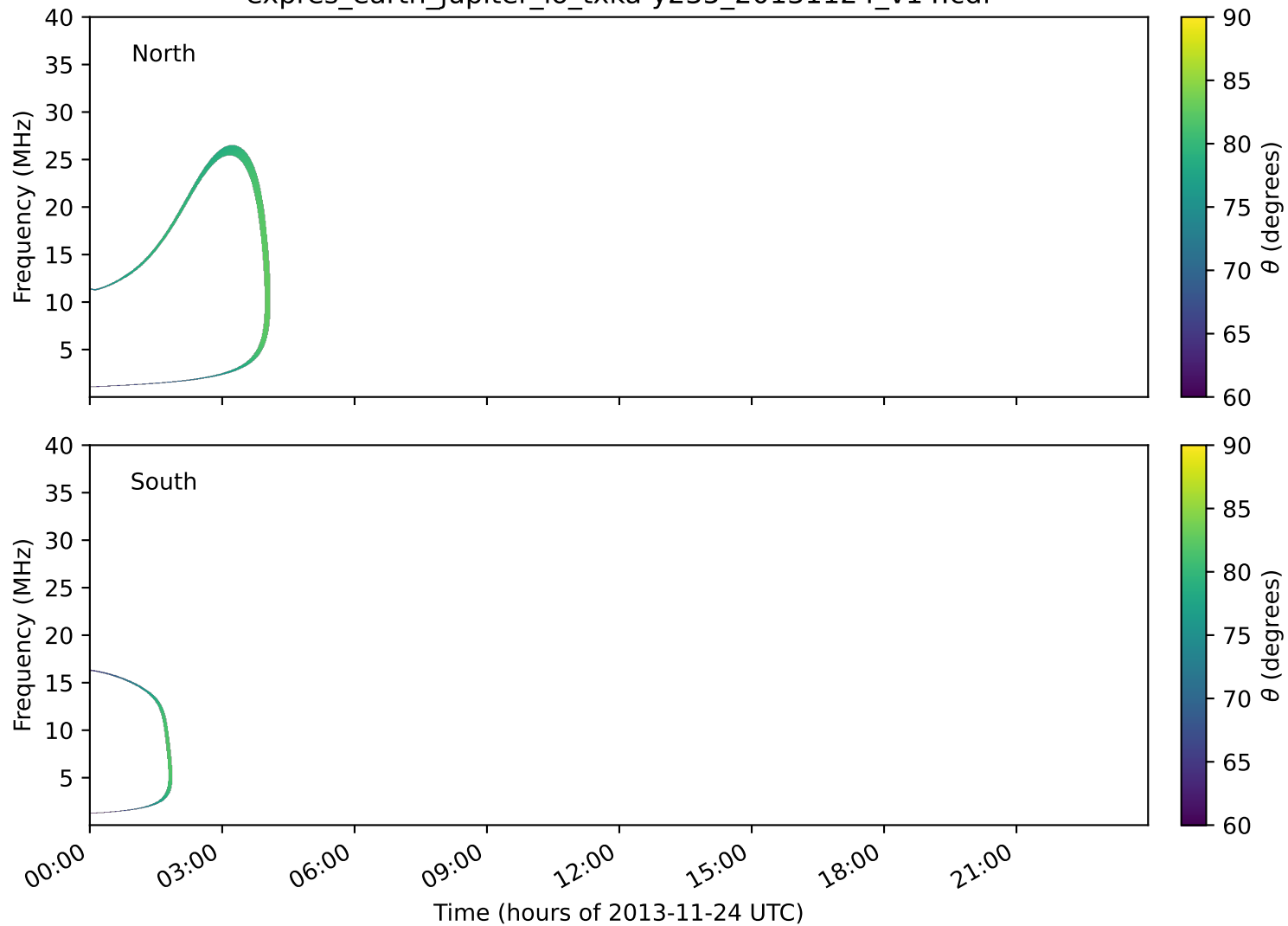
expres_earth_jupiter_io_txka-y235_20131124_v14.cdf
