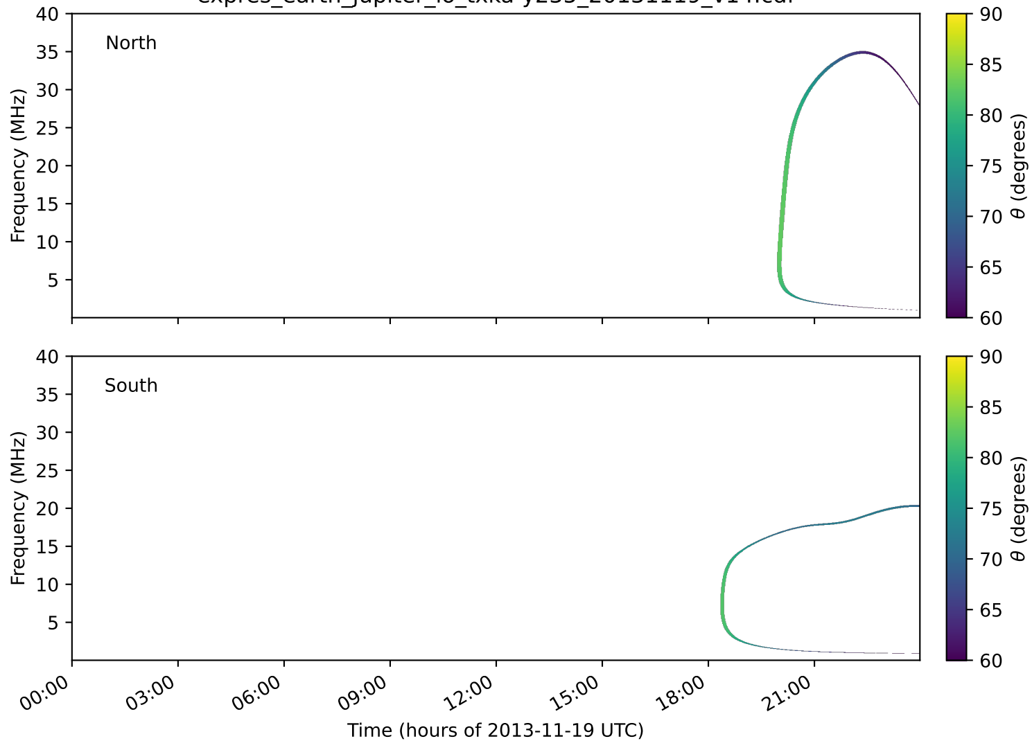
expres_earth_jupiter_io_txka-y235_20131119_v14.cdf
