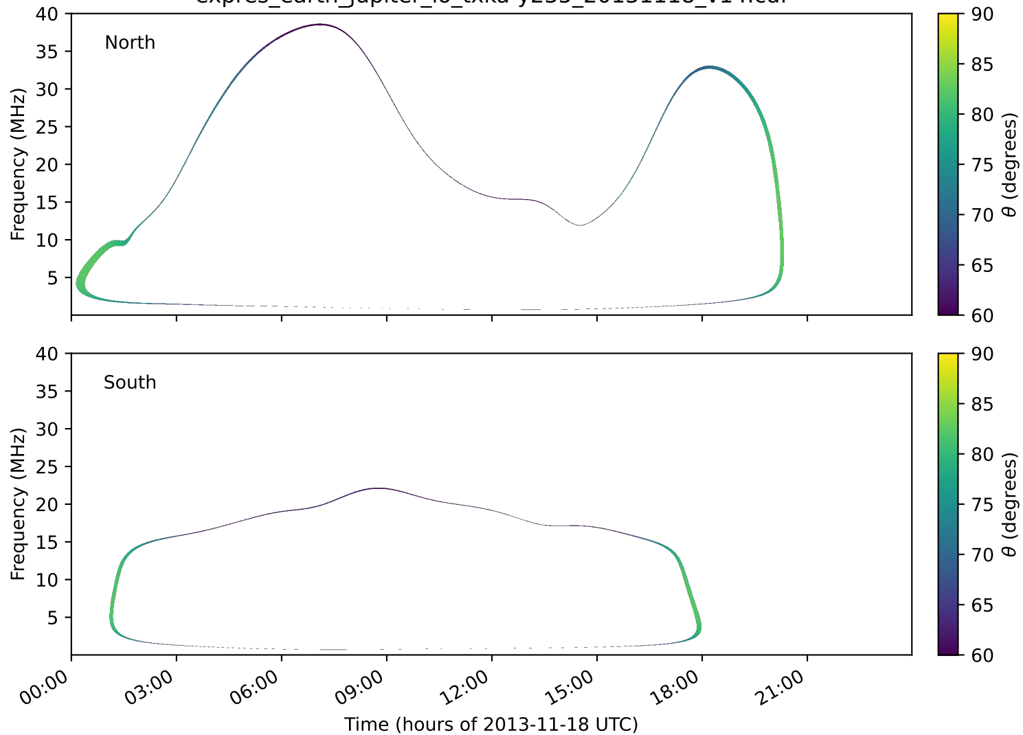
expres_earth_jupiter_io_txka-y235_20131118_v14.cdf
