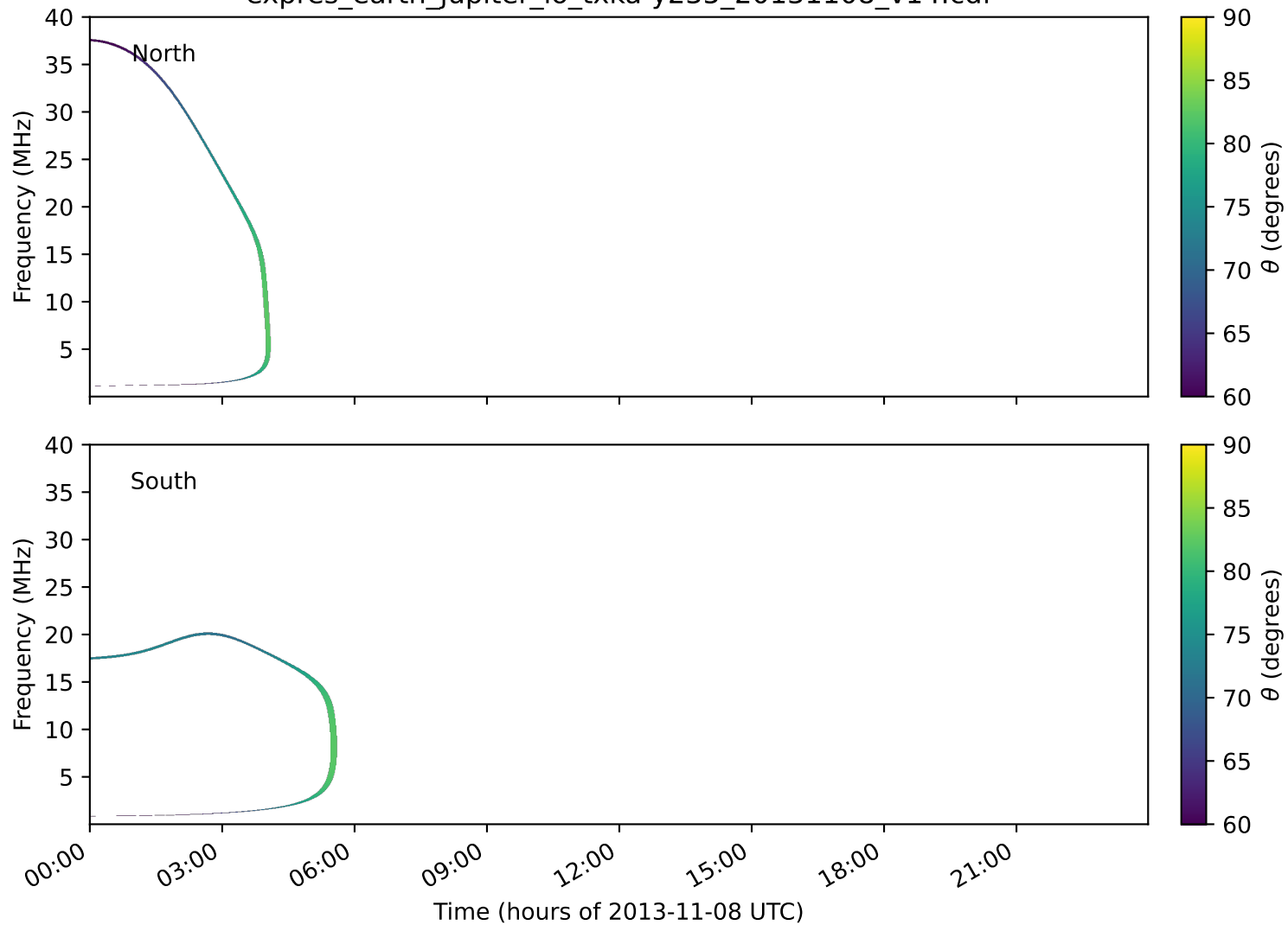
expres_earth_jupiter_io_txka-y235_20131108_v14.cdf
