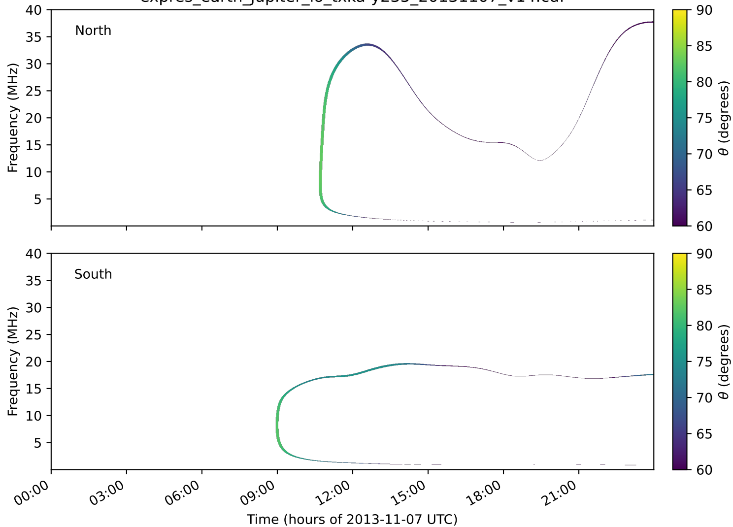
expres_earth_jupiter_io_txka-y235_20131107_v14.cdf
