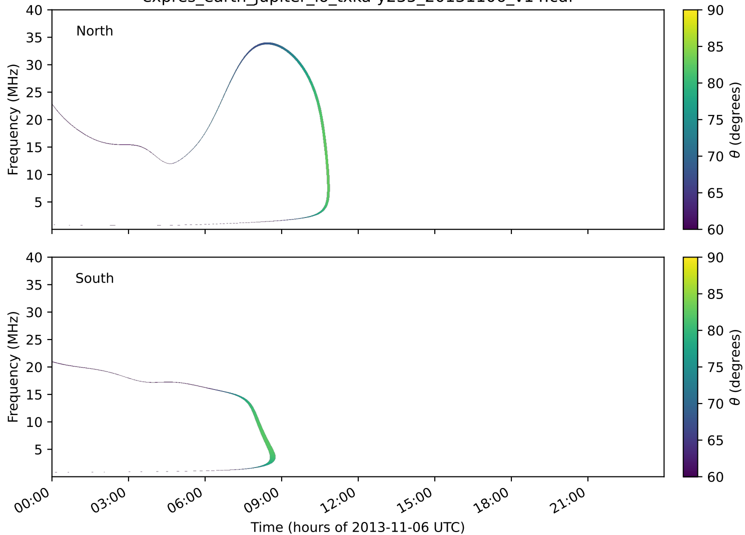
expres_earth_jupiter_io_txka-y235_20131106_v14.cdf
