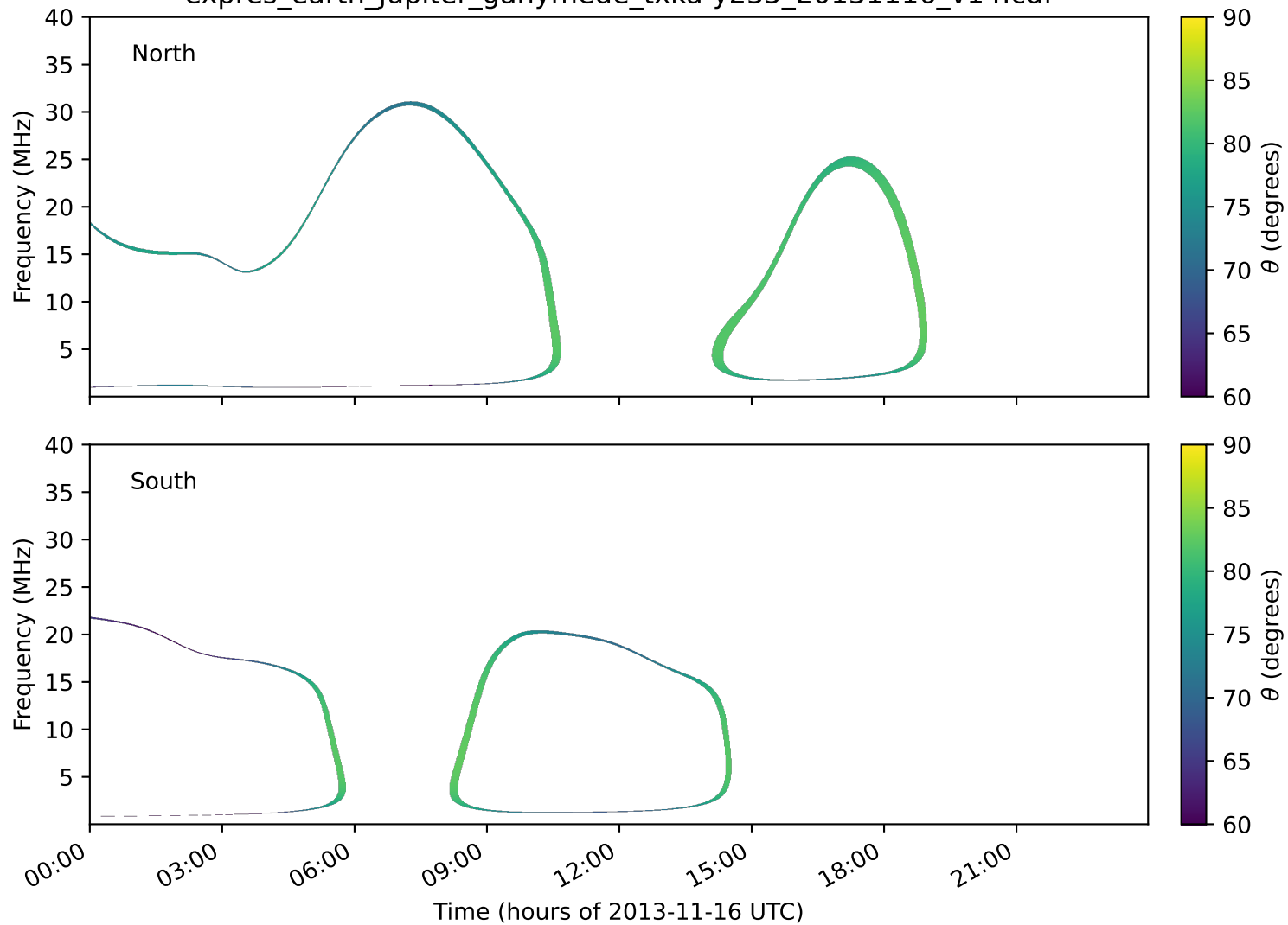
expres_earth_jupiter_ganymede_txka-y235_20131116_v14.cdf
