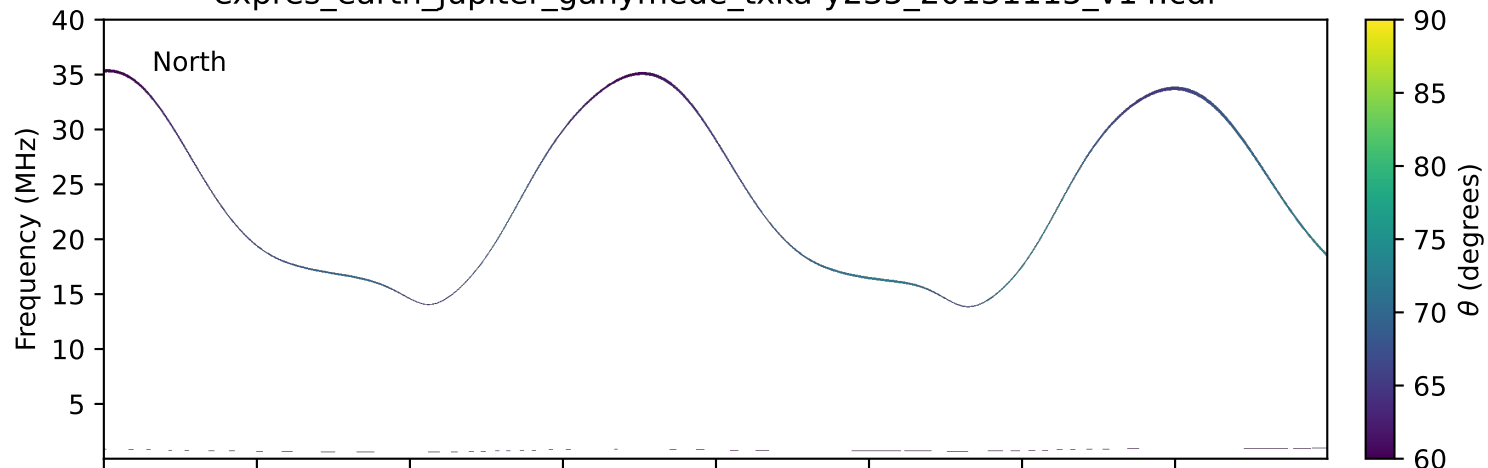
expres_earth_jupiter_ganymede_txka-y235_20131115_v14.cdf
