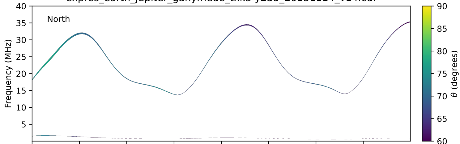
expres_earth_jupiter_ganymede_txka-y235_20131114_v14.cdf
