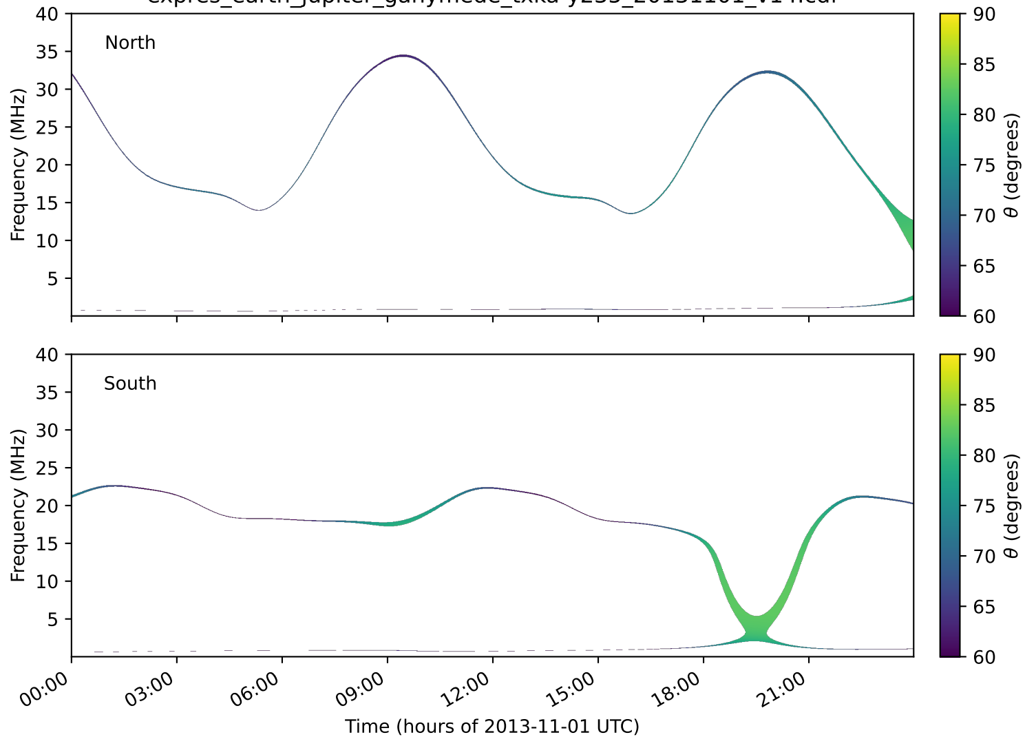
expres_earth_jupiter_ganymede_txka-y235_20131101_v14.cdf
