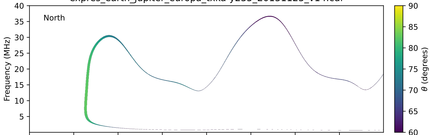
expres_earth_jupiter_europa_txka-y235_20131123_v14.cdf
