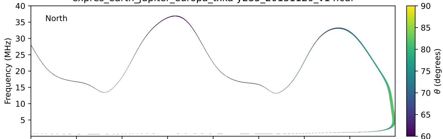
expres_earth_jupiter_europa_txka-y235_20131120_v14.cdf
