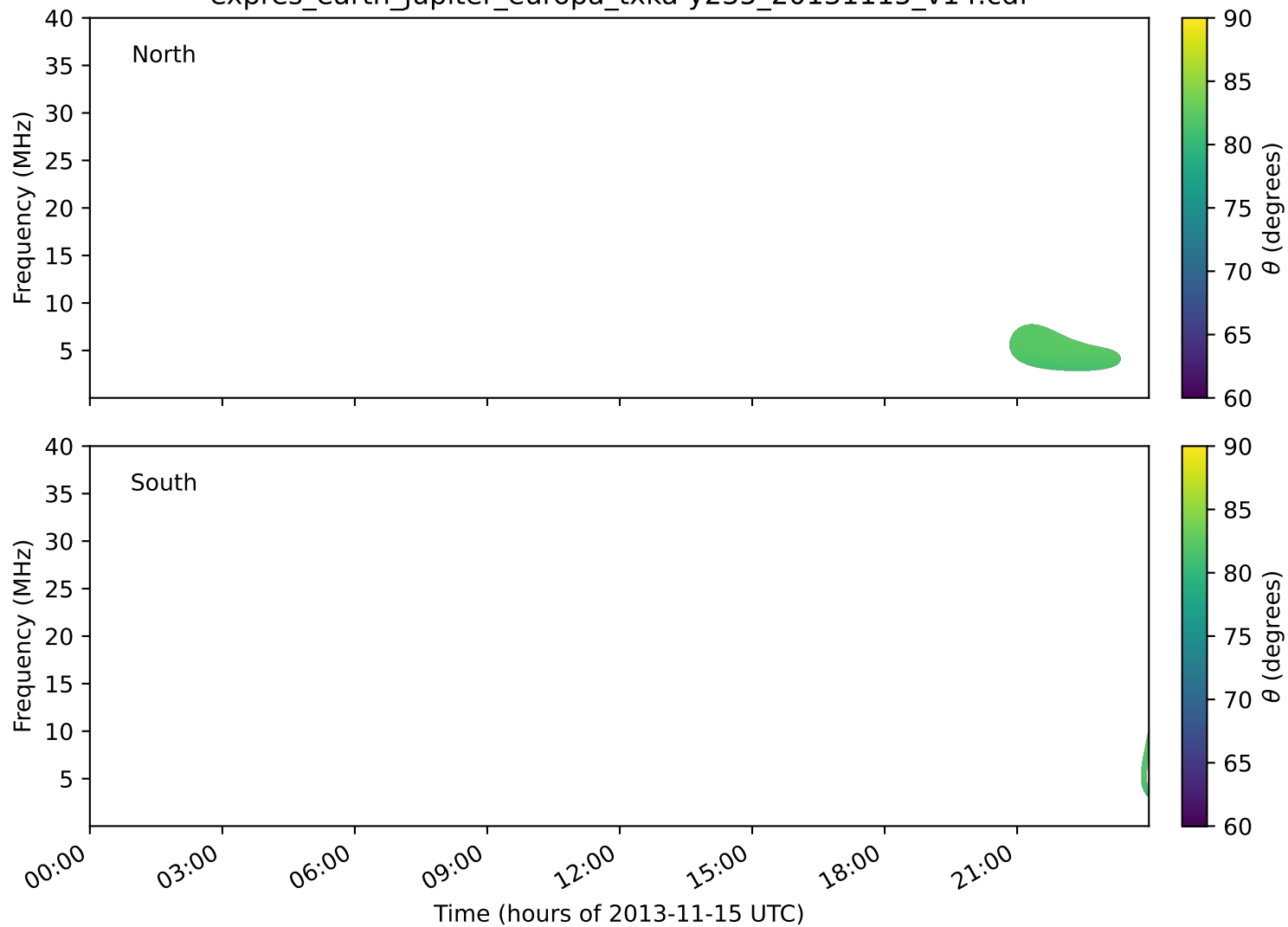
expres_earth_jupiter_europa_txka-y235_20131115_v14.cdf
