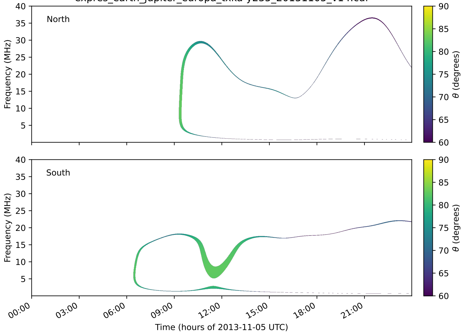
expres_earth_jupiter_europa_txka-y235_20131105_v14.cdf
