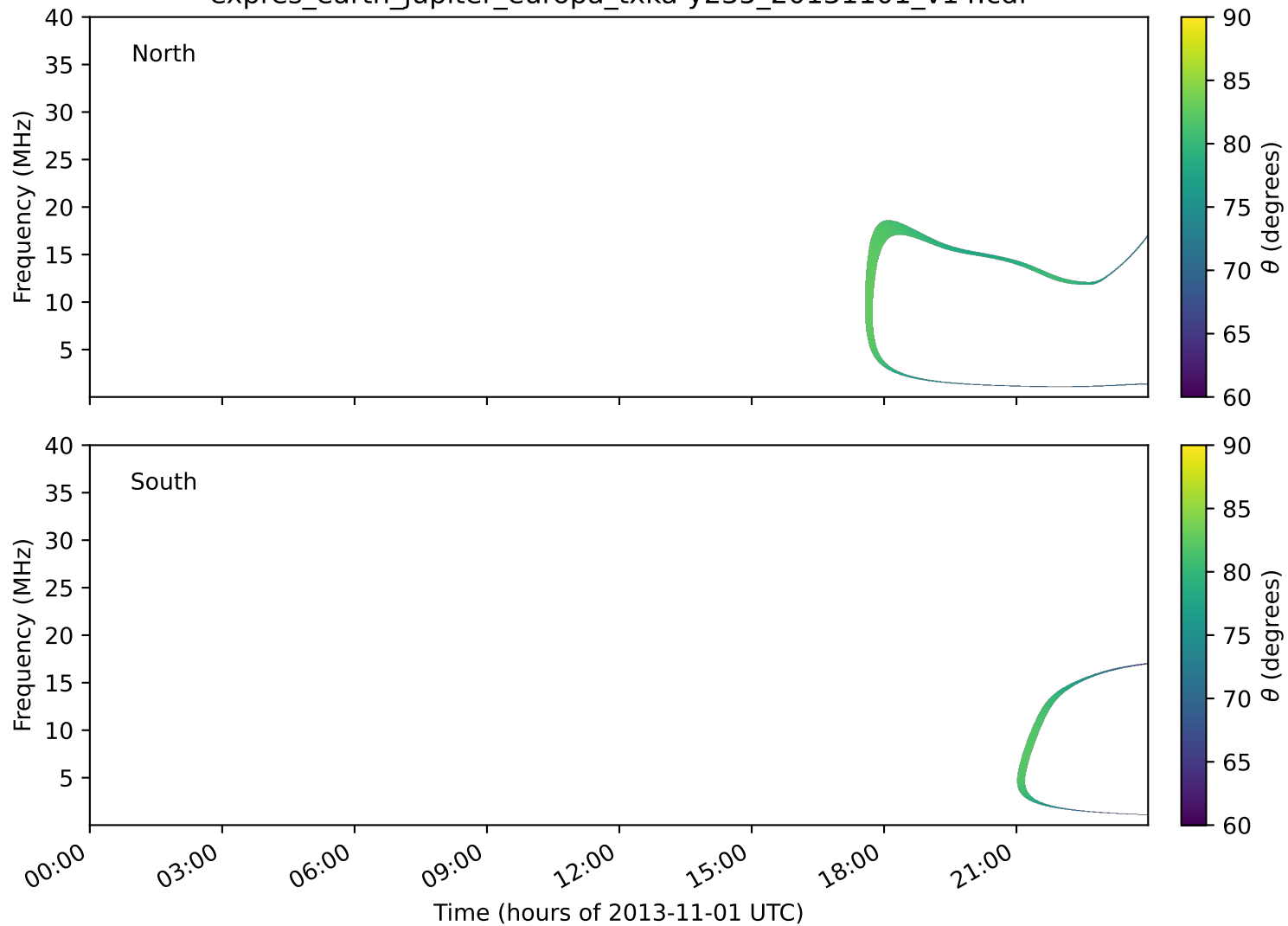
expres_earth_jupiter_europa_txka-y235_20131101_v14.cdf
