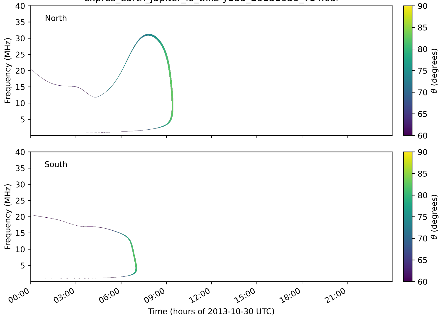
expres_earth_jupiter_io_txka-y235_20131030_v14.cdf
