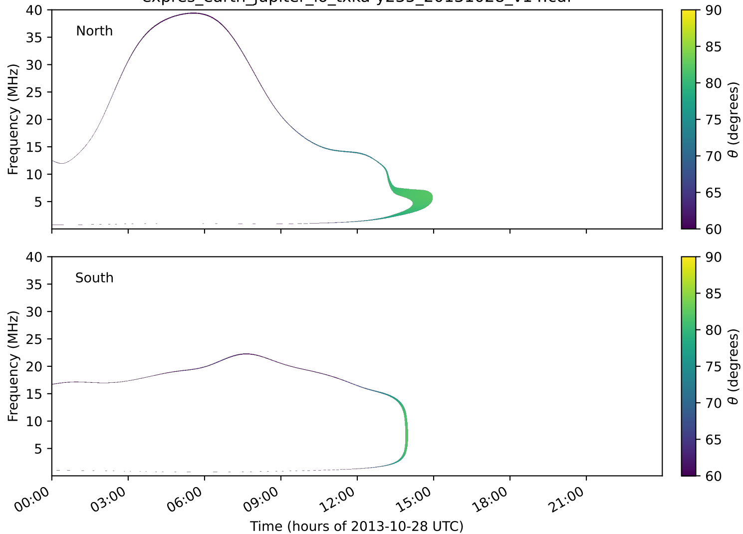
expres_earth_jupiter_io_txka-y235_20131028_v14.cdf
