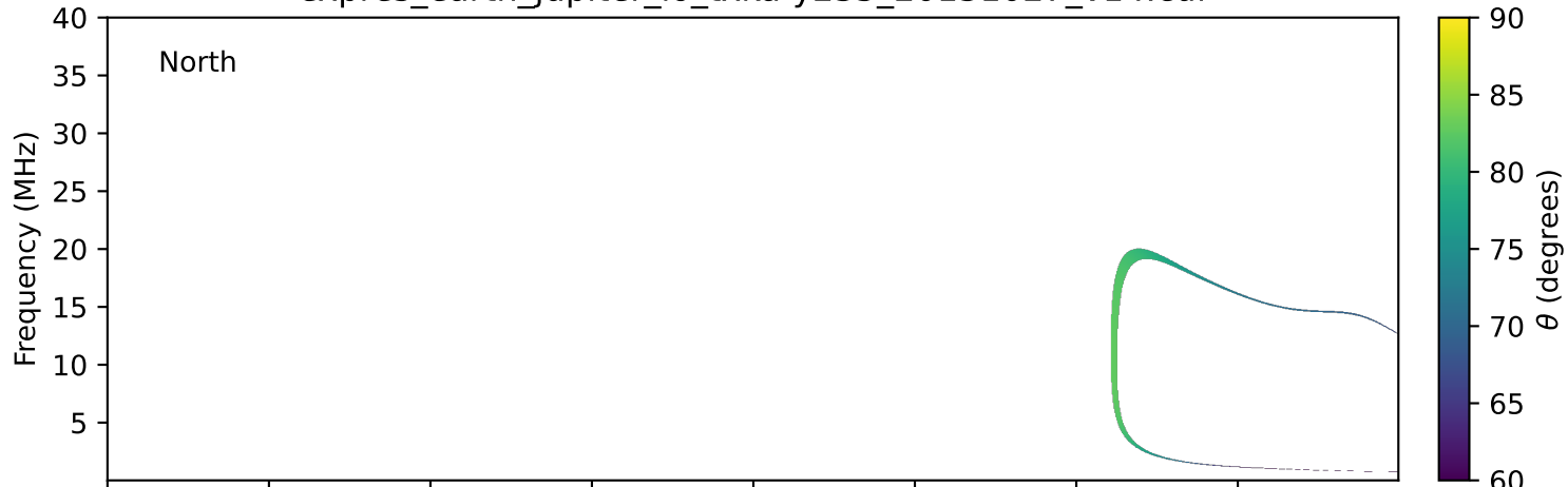
expres_earth_jupiter_io_txka-y235_20131027_v14.cdf
