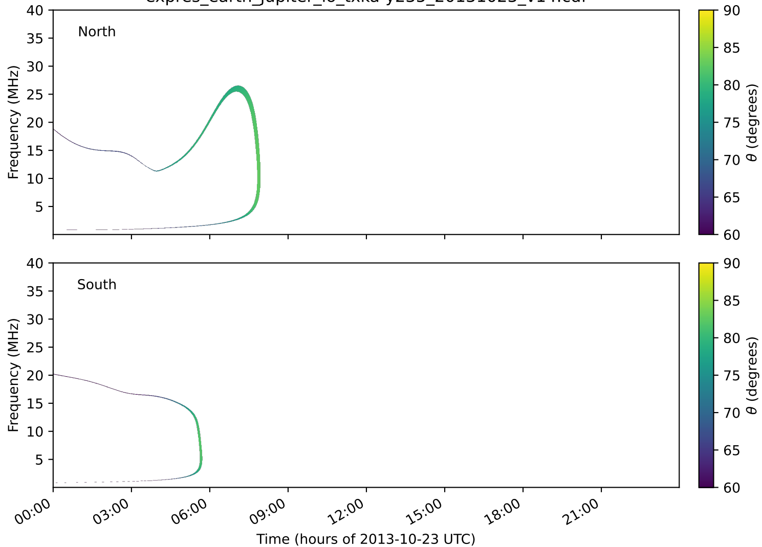
expres_earth_jupiter_io_txka-y235_20131023_v14.cdf
