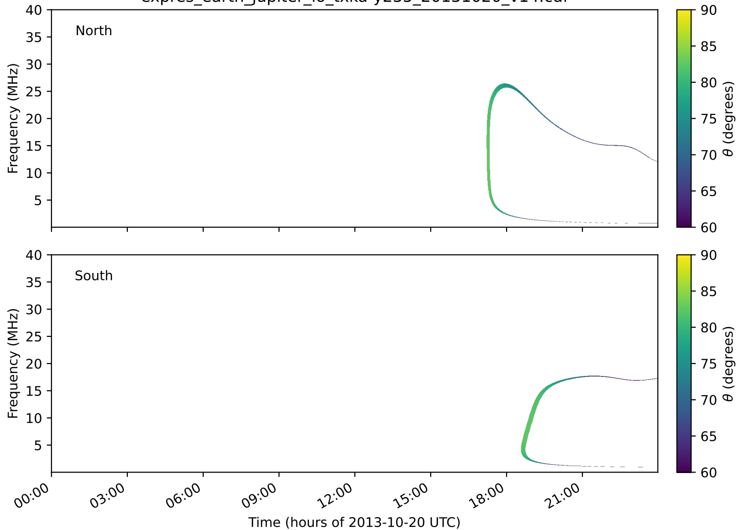
expres_earth_jupiter_io_txka-y235_20131020_v14.cdf
