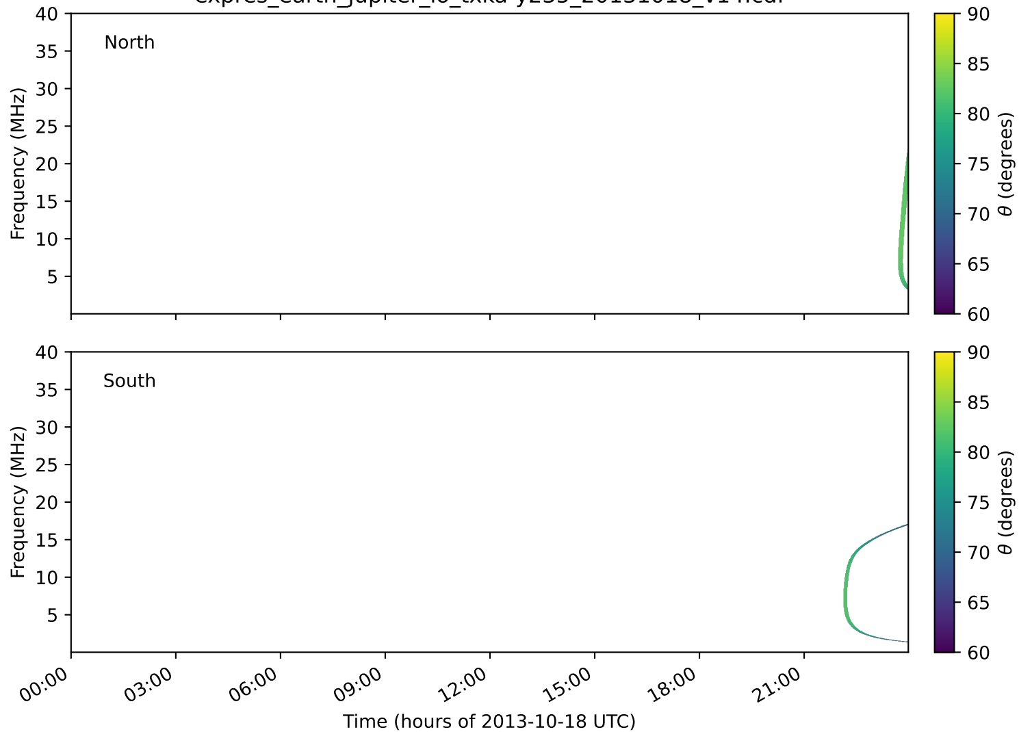
expres_earth_jupiter_io_txka-y235_20131018_v14.cdf
