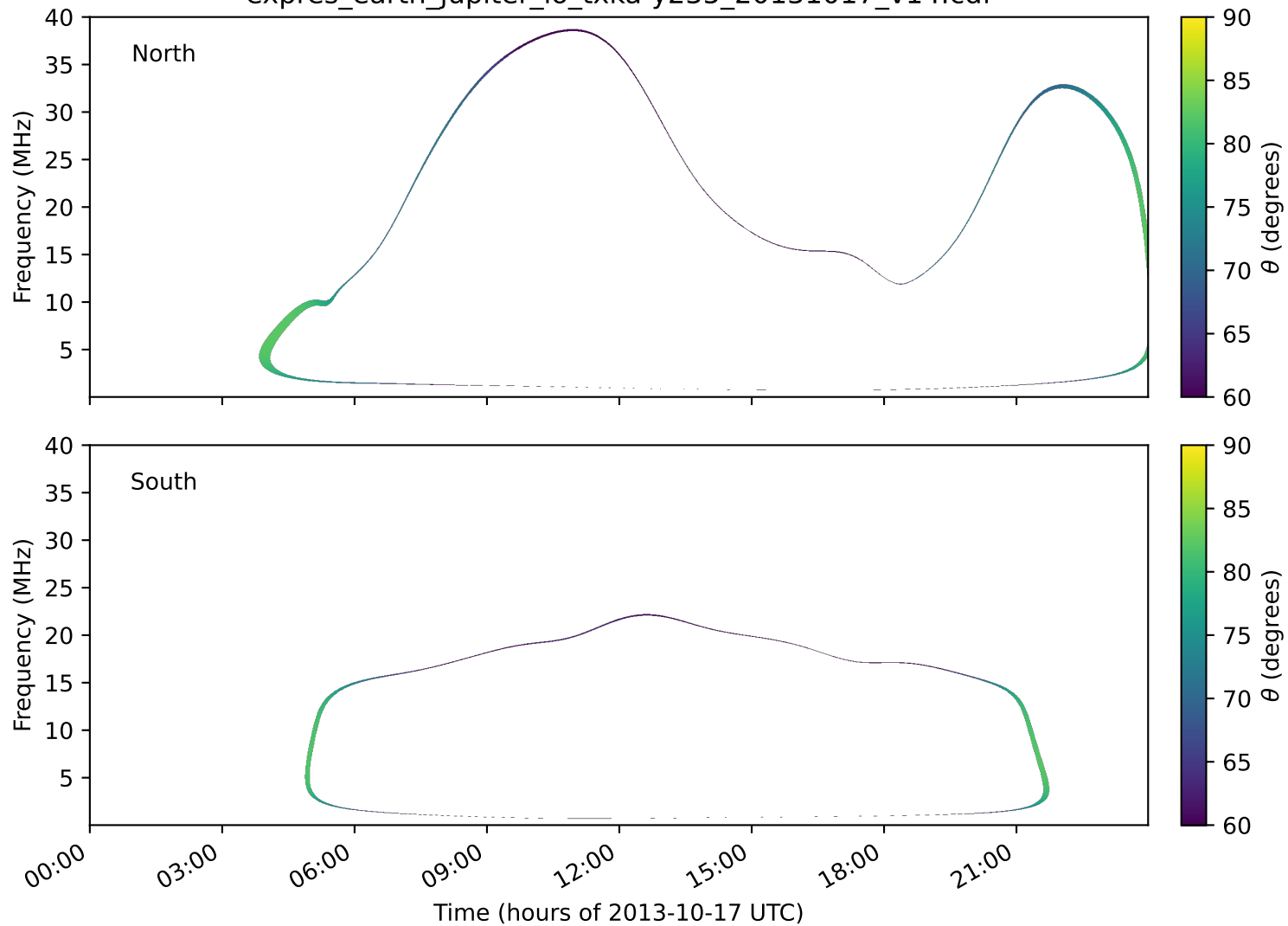
expres_earth_jupiter_io_txka-y235_20131017_v14.cdf
