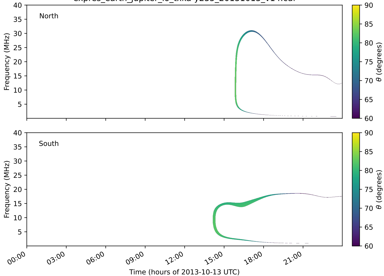
expres_earth_jupiter_io_txka-y235_20131013_v14.cdf
