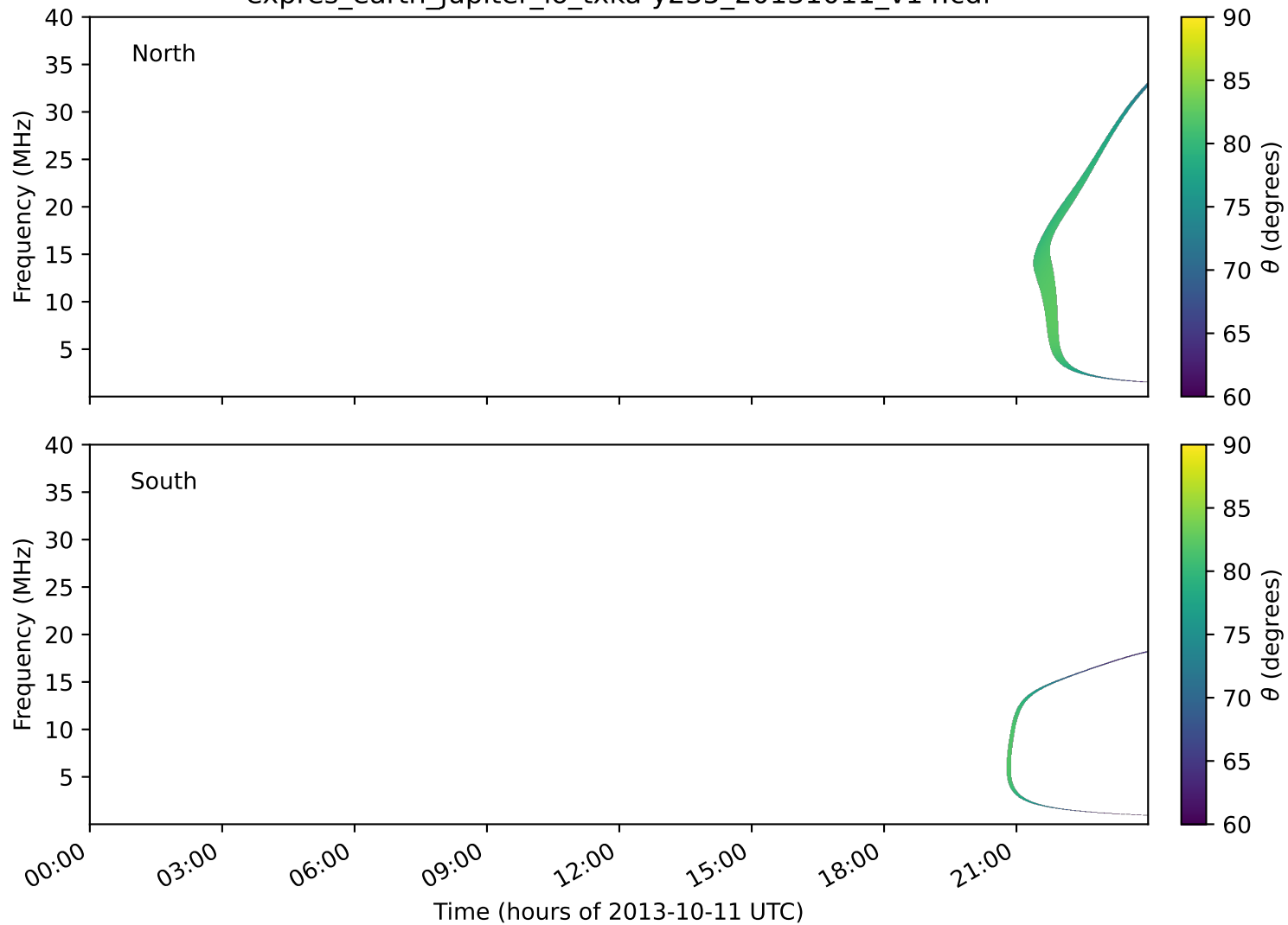
expres_earth_jupiter_io_txka-y235_20131011_v14.cdf
