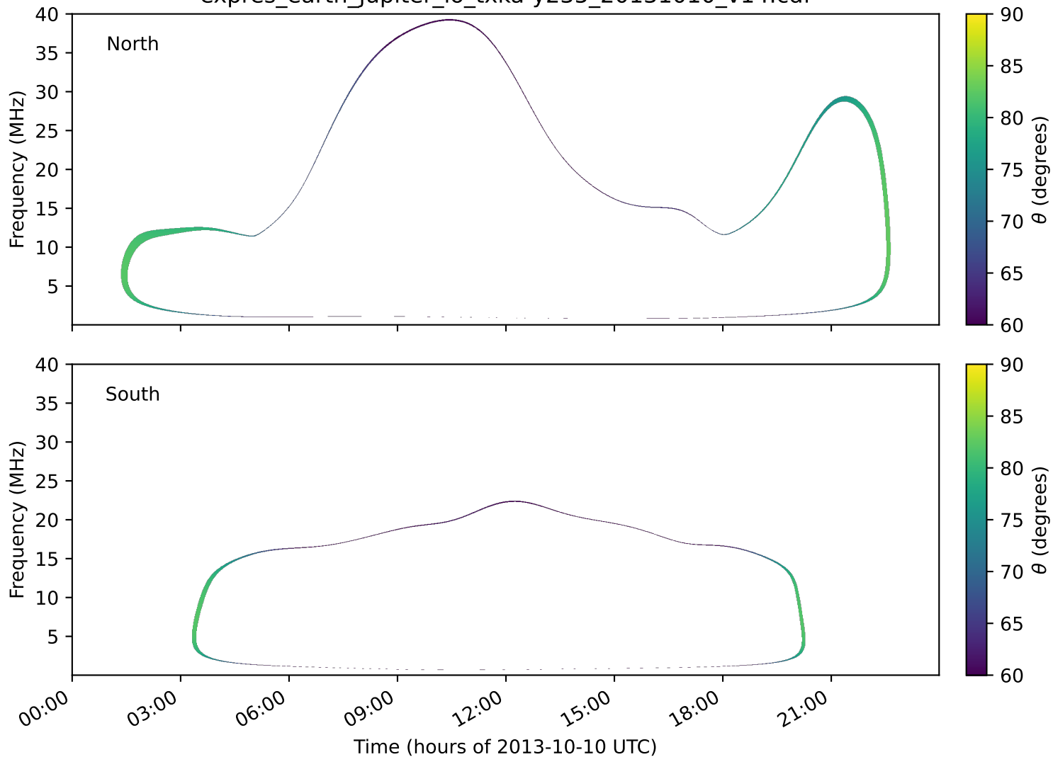
expres_earth_jupiter_io_txka-y235_20131010_v14.cdf
