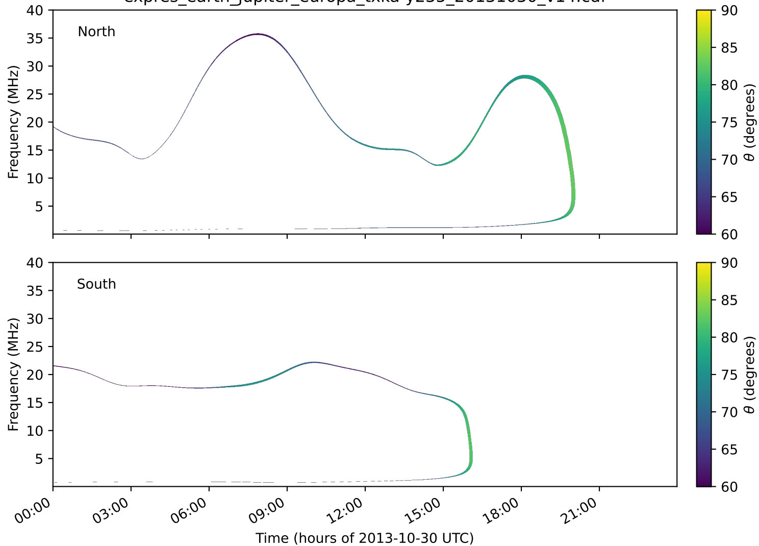
expres_earth_jupiter_europa_txka-y235_20131030_v14.cdf
