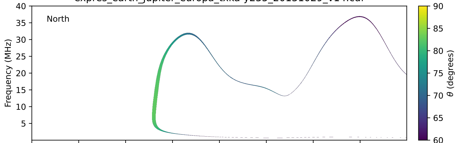
expres_earth_jupiter_europa_txka-y235_20131029_v14.cdf
