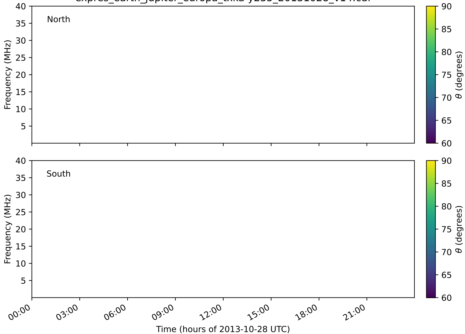
expres_earth_jupiter_europa_txka-y235_20131028_v14.cdf
