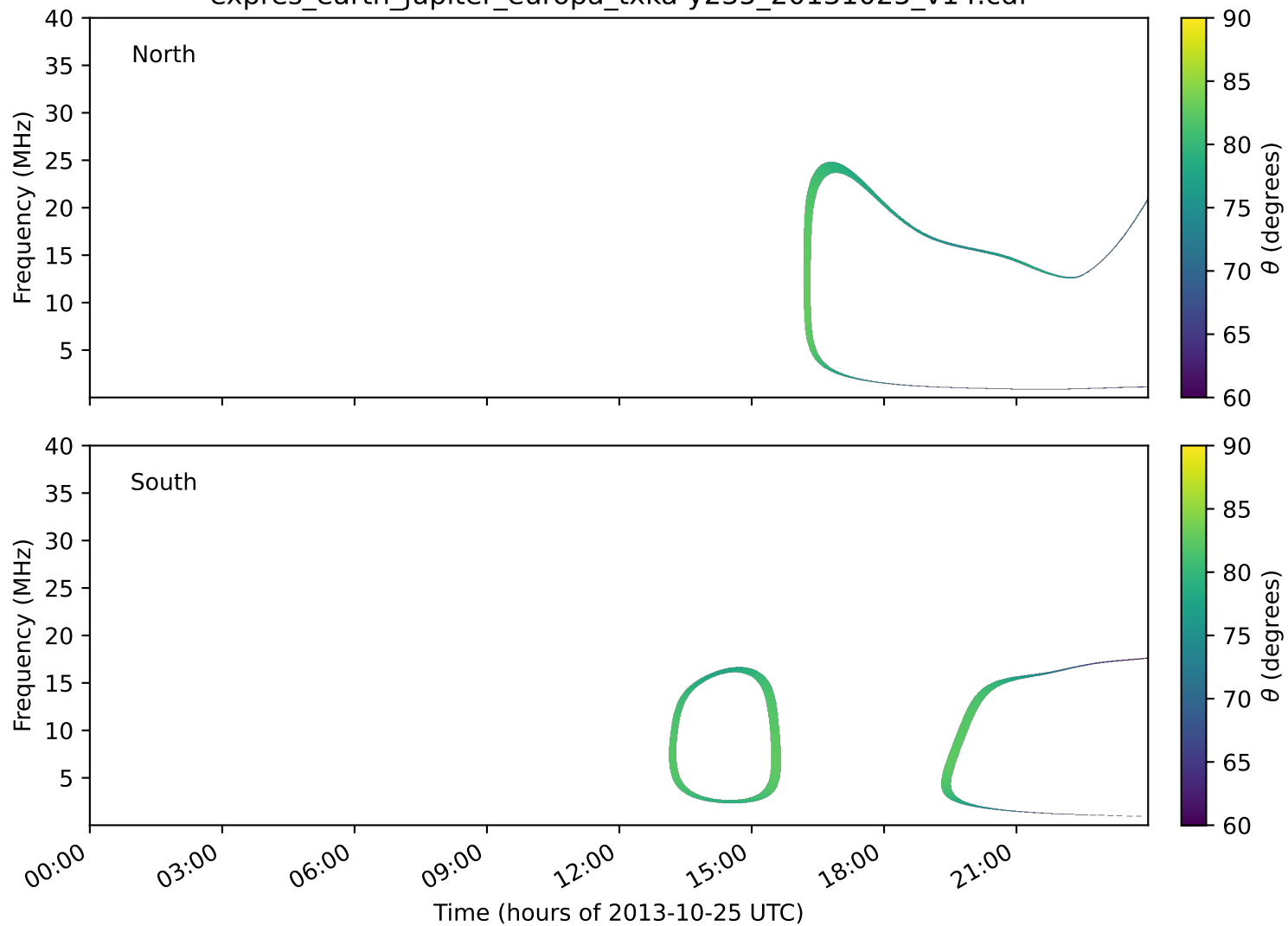
expres_earth_jupiter_europa_txka-y235_20131025_v14.cdf
